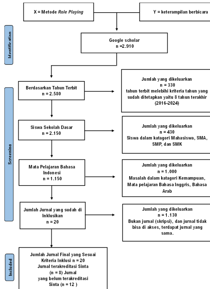
Gambar 1 Diagram PRISMA
